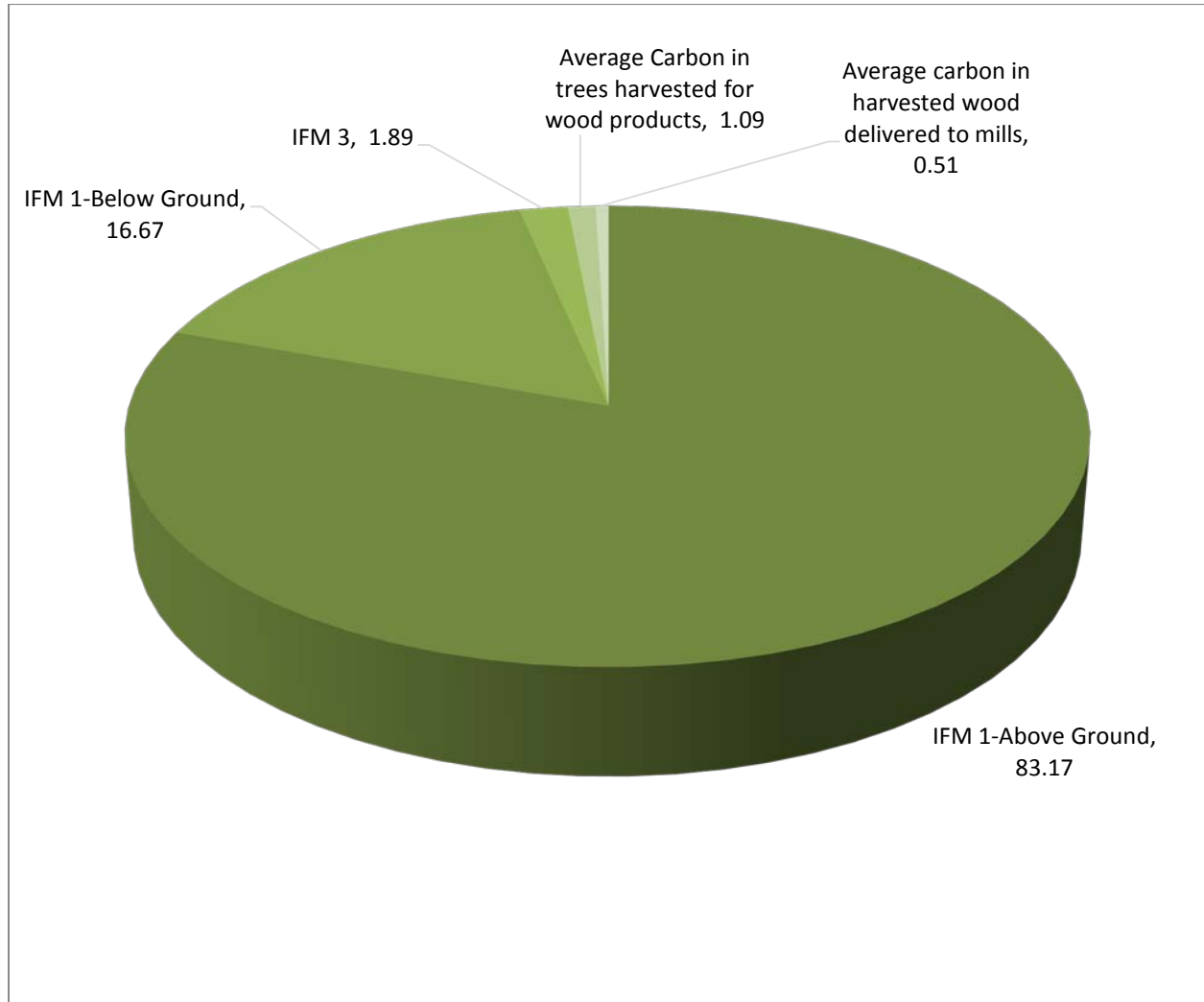
Figure 2. Final Baseline Carbon Stocks (tCO 2 e/acre)
