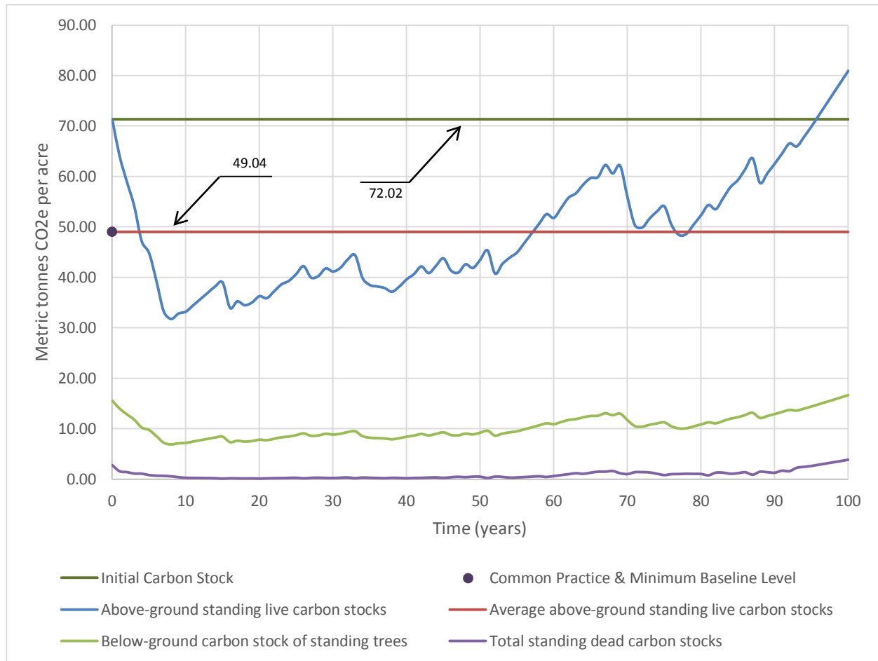
Figure 1. Baseline Onsite Carbon Stocks over 100 years
