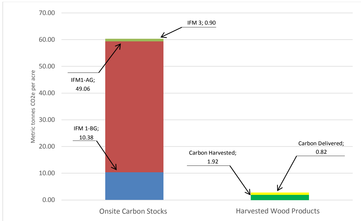
Figure 2. Average Baseline Carbon Stocks: Onsite Carbon Stocks and Harvested Wood Products (tCO 2 e/acre)
