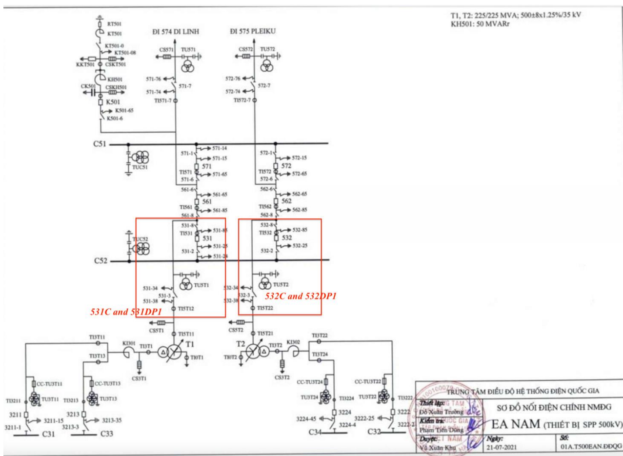
Figure 5 – Single Line Diagram of Ea Nam WPP
