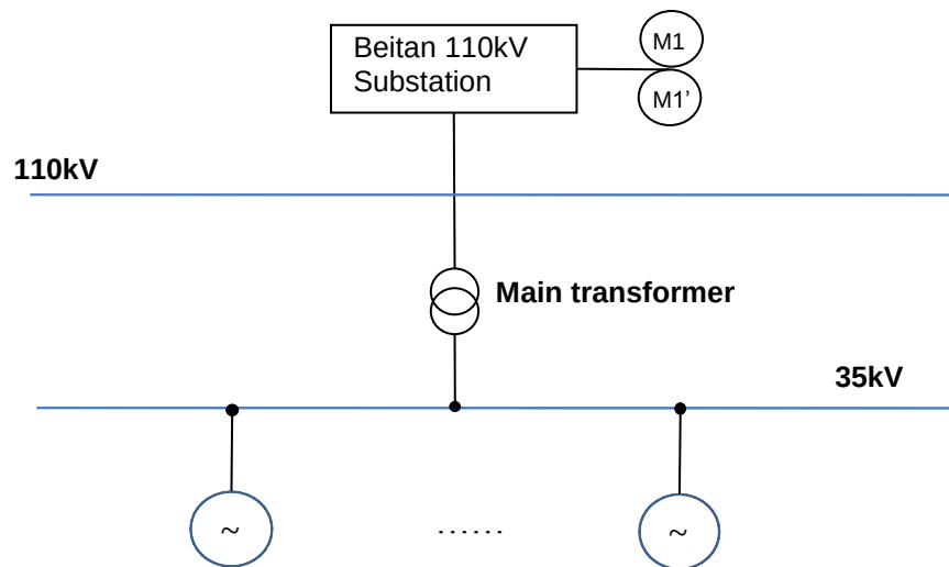
Figure 5: Power line diagram of the monitoring system
