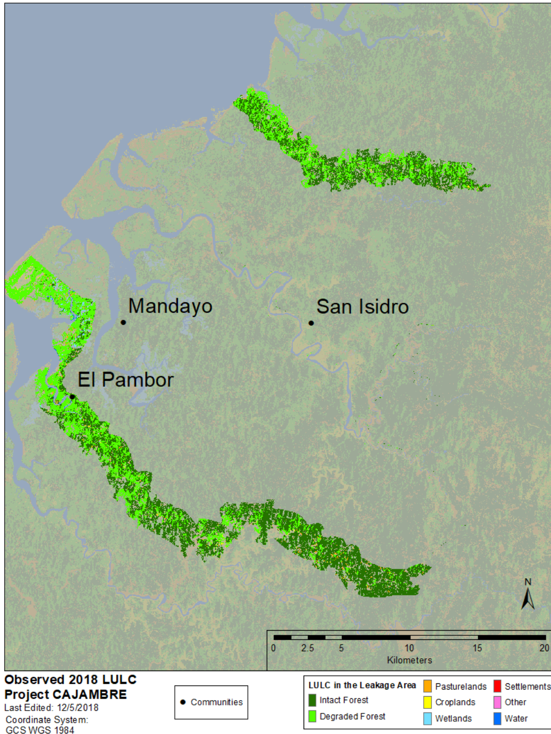
Figure 3: LULC Classification in Leakage Area
