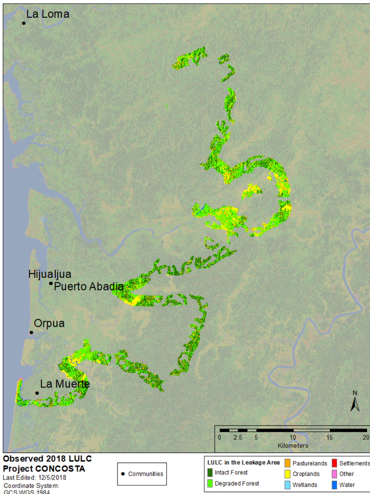
Figure 3: LULC Classification in Leakage Area
