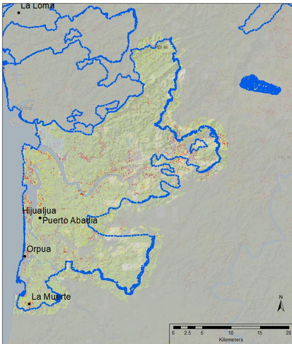
Figure 5: LULC Transitions 2012-2018 in Project Area and Leakage areas
