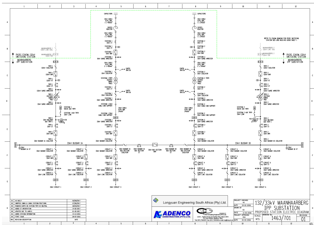
Figure 4.3-1: 132/33kV Maanhaarberg IPP Substation. Single Line Diagram
