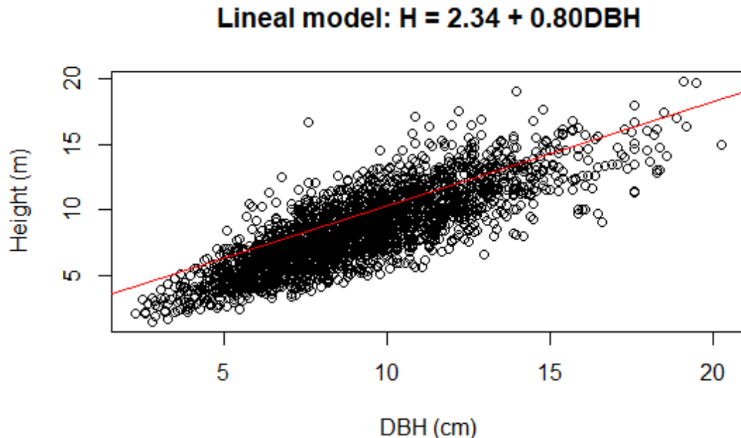
Figure 3. Distribution of the height-DBH data and model
