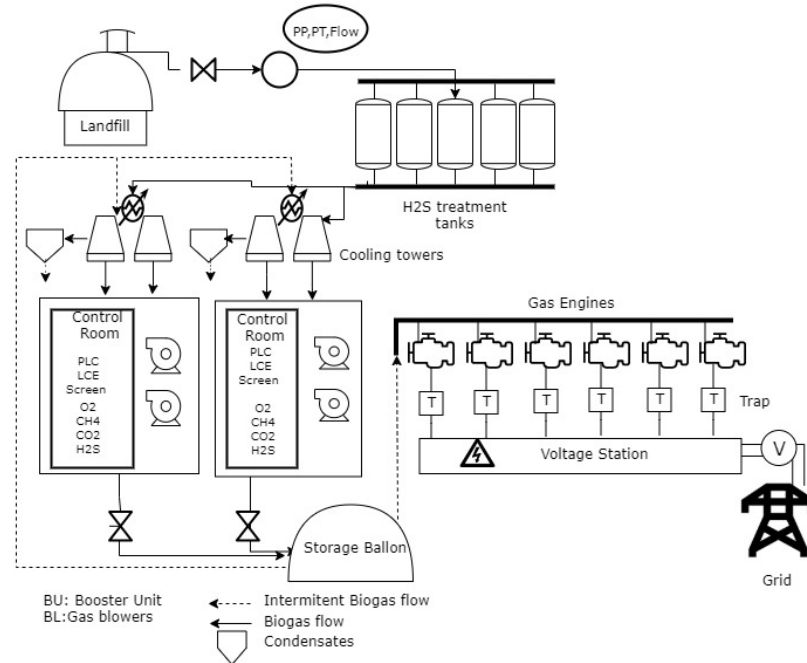
Figure 1. Flow Process Chart for the İzmir LFG Facility
