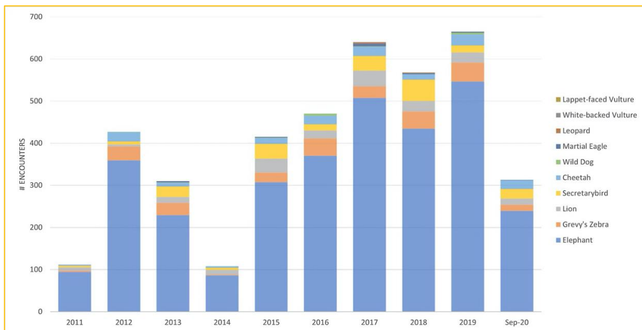
Figure 34: Total number of encounters of the key HCV species recorded by the Wildlife Works' rangers on patrol across KCRPII from 2011 to the 2020 reporting period.
