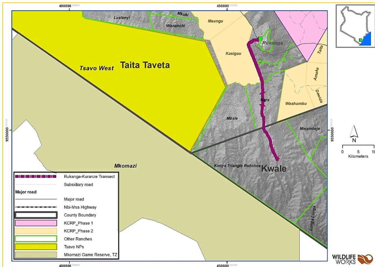
Figure 42: Rukanga-Kuranze road transect shown with the KCRPII Project Area, Tsavo West National Park and the Kenya-Tanzania border.
