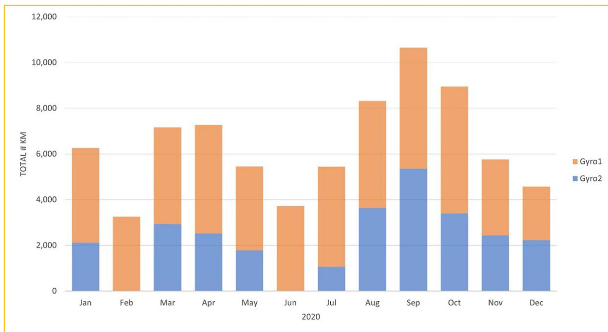
Figure 36: Monthly distances covered by the two resident gyrocopters traversing the KCRPII during the 2020 reporting period.
