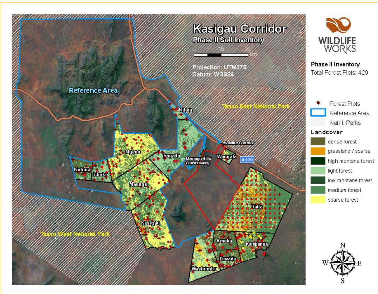
Figure 10: All Biomass sample plot locations in Kasigau Corridor REDD+ Project Phase II Project Ar
