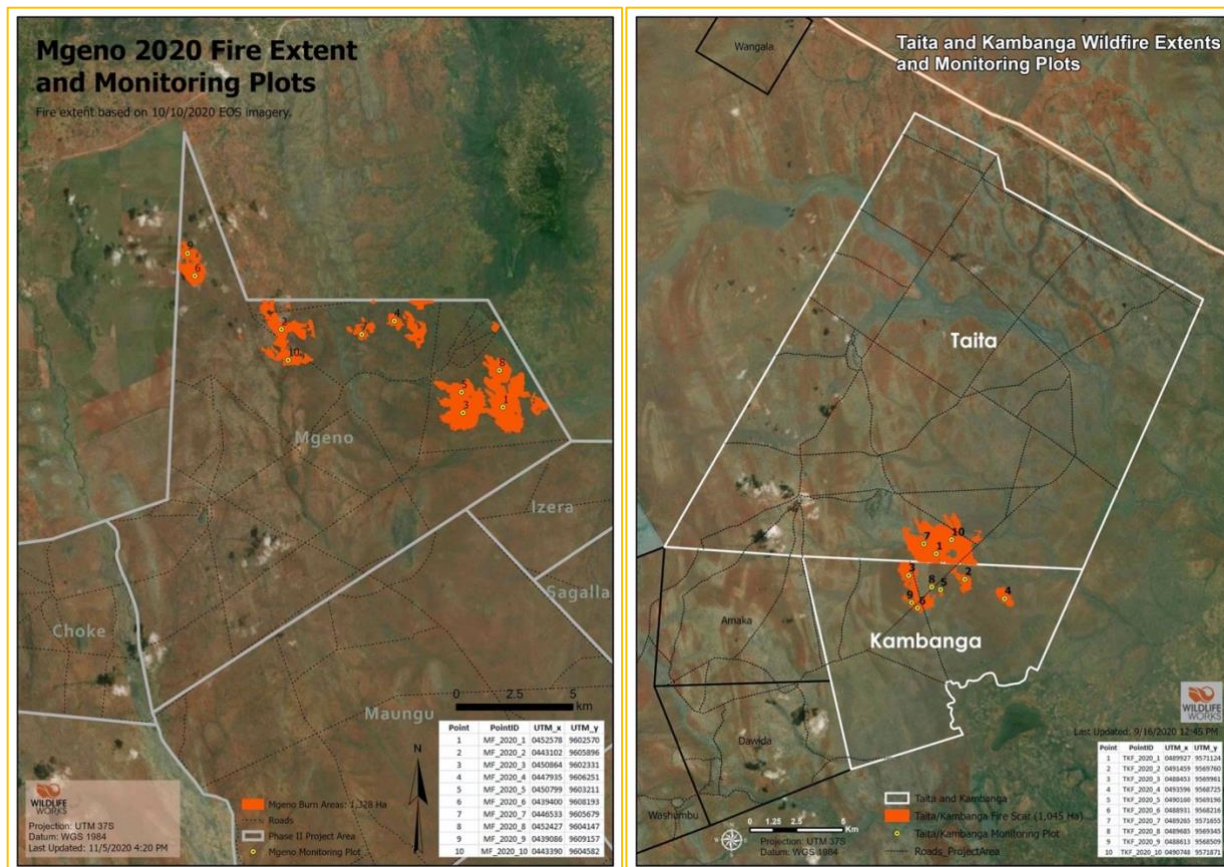
Figure 12: The extent of the wildfires on Mgeno ranch and Taita and Kambanga ranches, and the location of forest sampling plots.
